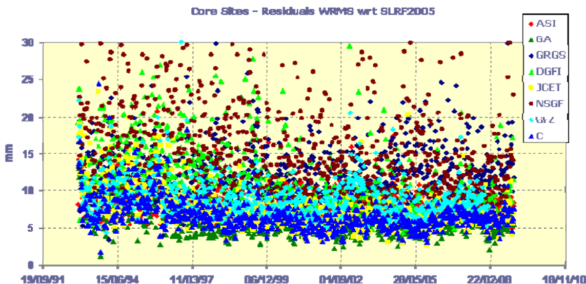
Figure 8. 3D wrms of the core site coordinates residuals with respect to SLRF2005.
